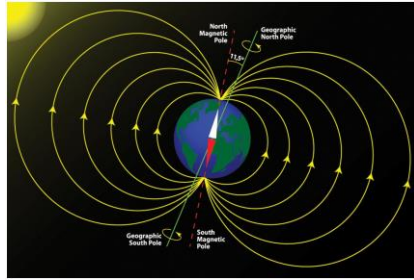
Fig 1: Curved Earth's geomagnetic field lines relative to the surface of the Earth [13]
