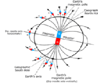
Fig 2: Close up depiction of the Earth's geomagnetic field lines [14]
