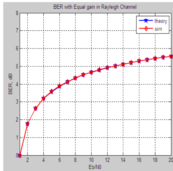
Figure 5. Equal gain combining in Rayleigh channel.
