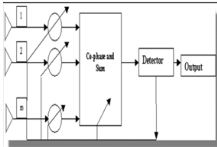
Figure2. Equal Gain Combining
