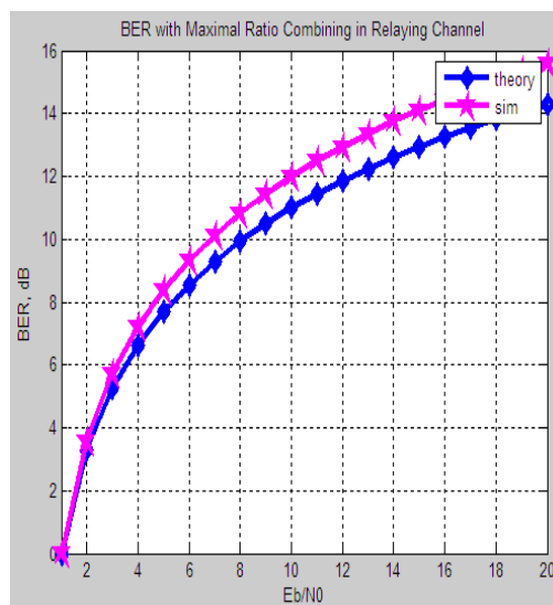
Figure 4. Maximal ratio combining in Rayleigh channel
