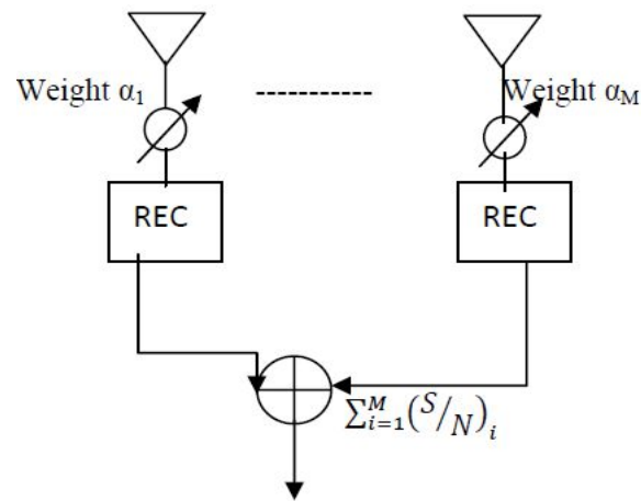
Figure1. Maximal Ratio Combining
