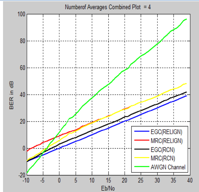
Figure 10. Comparison of Diversity techniques in different fading channels with respect to AWGN channel.
