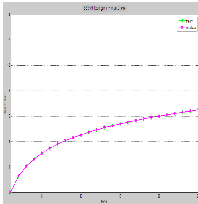
Figure 8. Equal Gain Combining in Rician channel.
