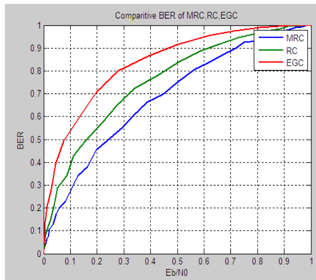
Figure 6. Comparison between Maximal ratio combining and Equal gain combining in Rayleigh channel.
