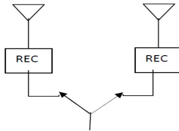
Figure3. Selection combining
