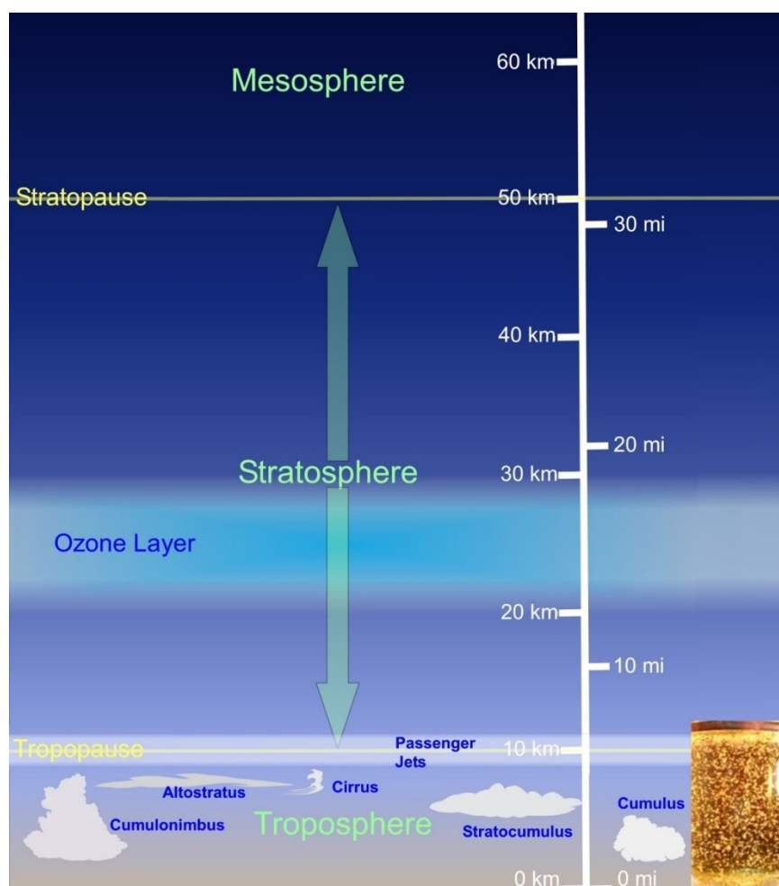
Figure 3. Schematic representation of the layers of Earth's atmosphere. The beaker-symbol in the lower right indicates the vertical region in which atmospheric convection takes place. From [26].
