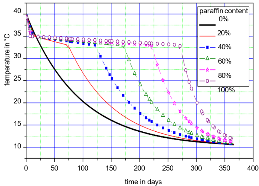
Figure 20: Cooling process of a water tank in dependence of the percentage of phase change materials (PCM) [4].
