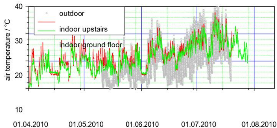
Figure 13: Profile of the outdoor and room air temperatures for the floating house “Ar-che” in the early summer and midsummer of 2010.
