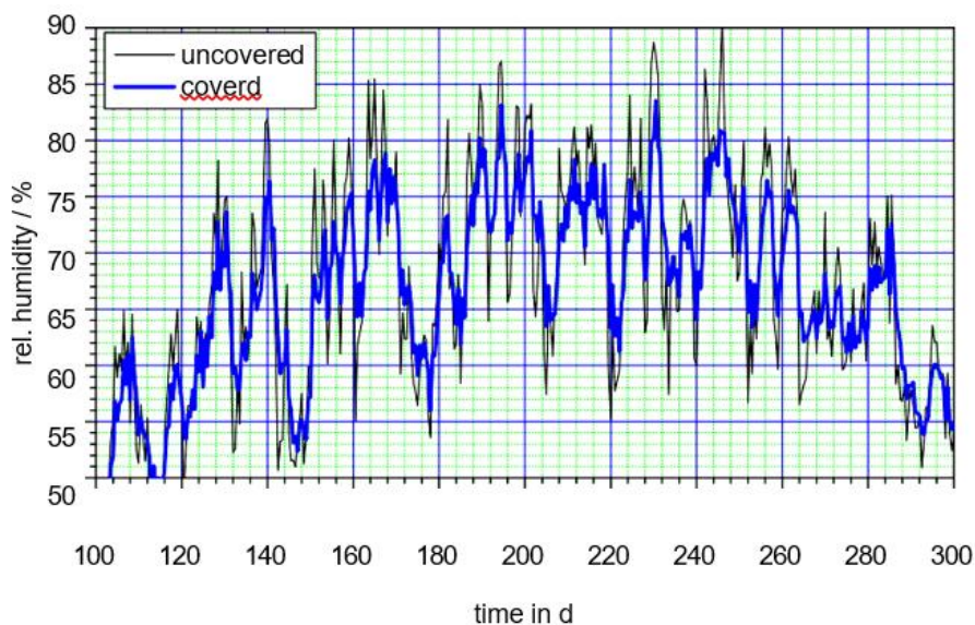
Figure 21: Comparison of the room air humidity between paneled and not panelled internal insulation made of foam glass.
